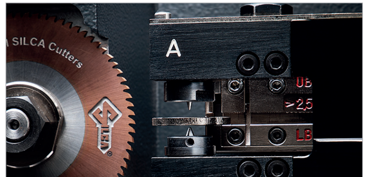
Engraving on both key sides (F900-F800-F600)
